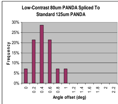
Fig. 5: LC 80 \mu m PANDA to 125 \mu m PANDA
